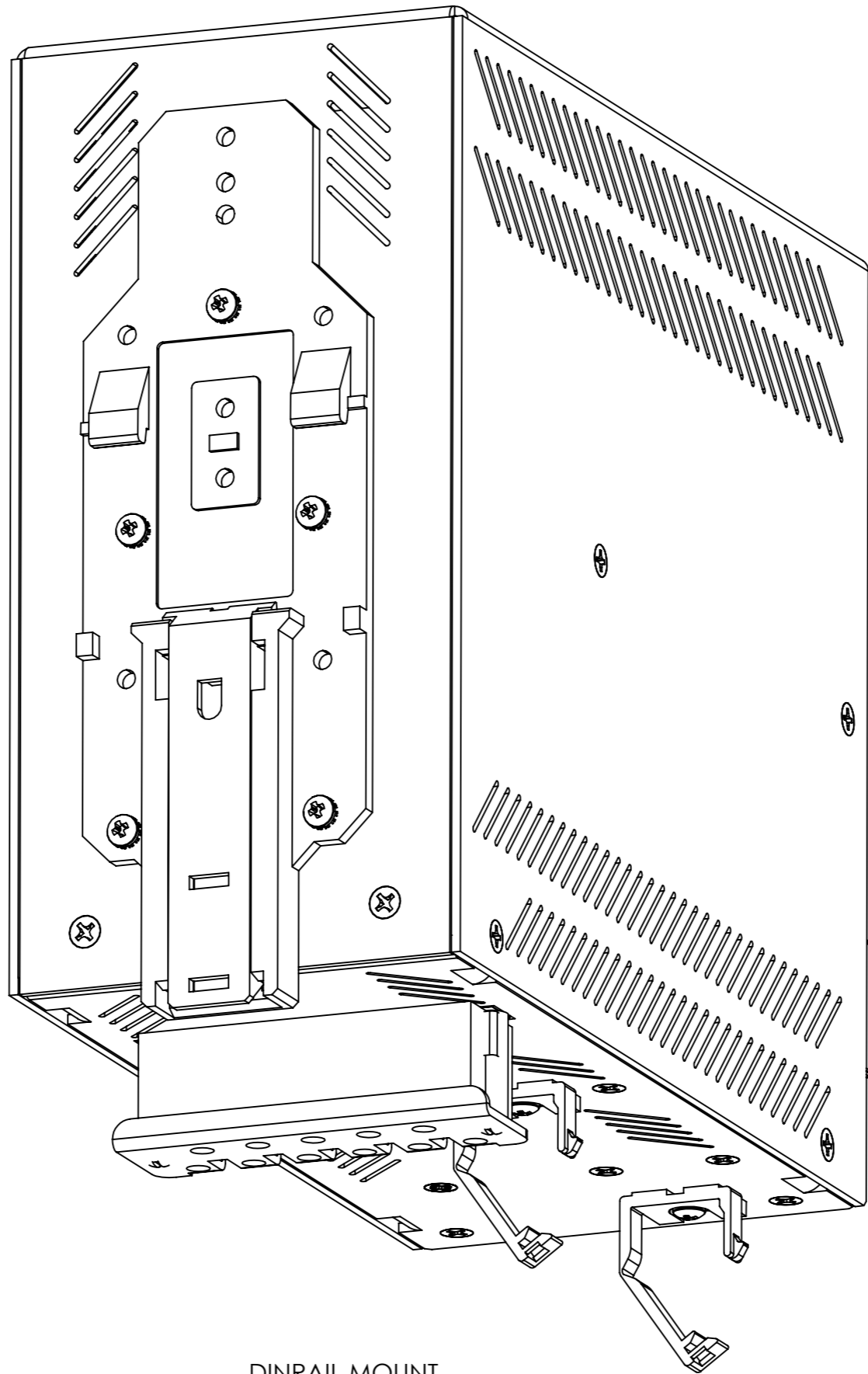
DINRAIL MOUNT
