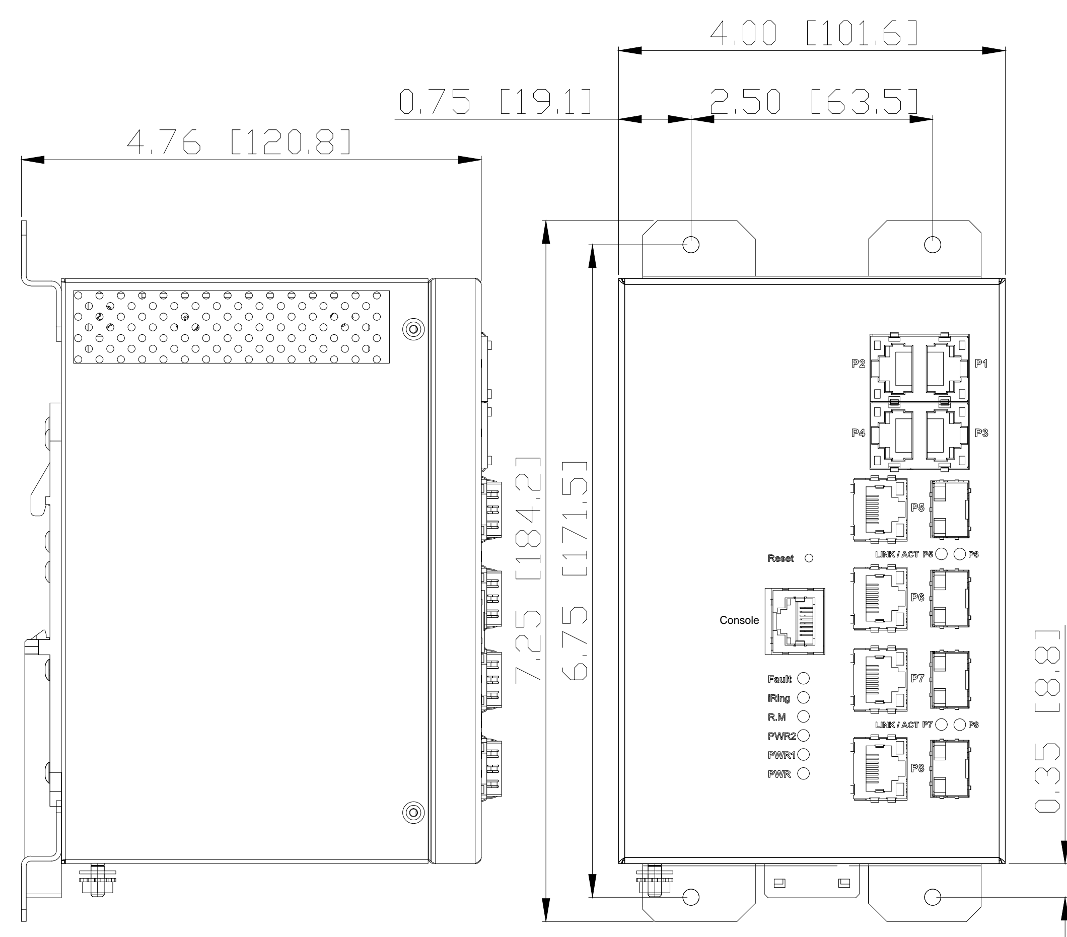
PANEL MOUNT BRACKET INSTALLED AT REAR
