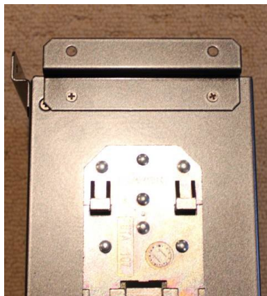
Figure 6 - Brackets Mounted on back of Switch
