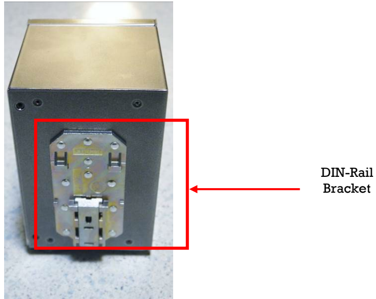
Figure 3 - DIN-Rail Bracket
