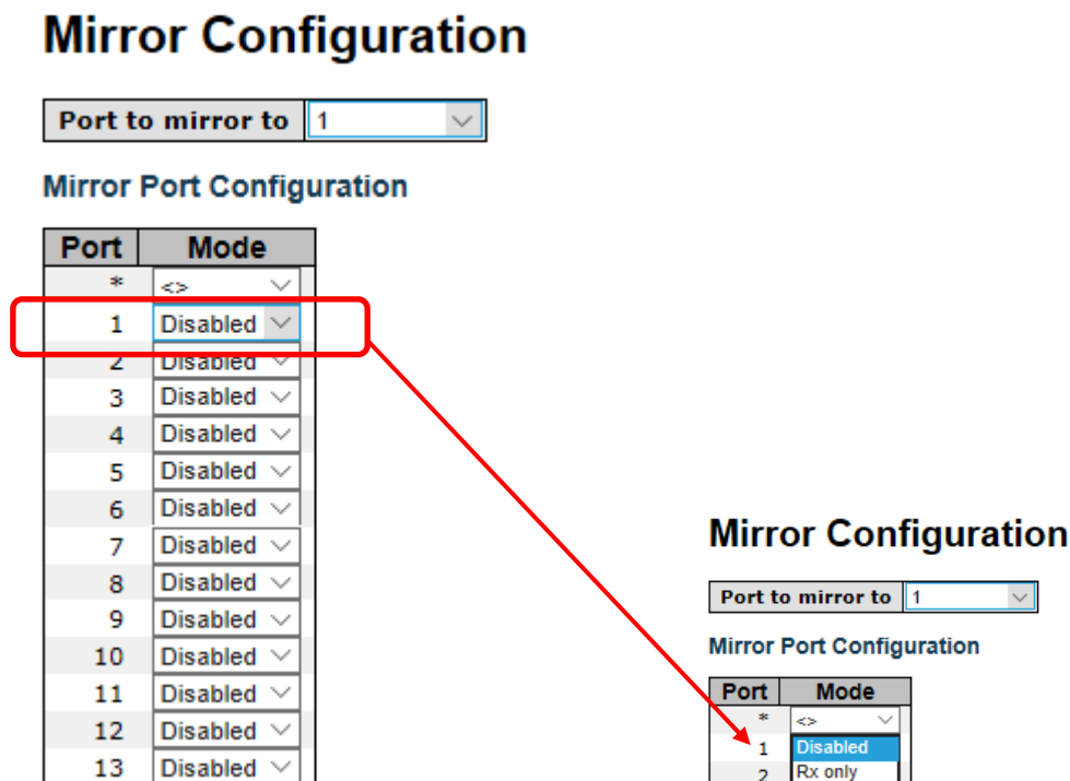
Figure 153 - Mirror Configuration
