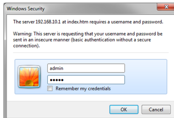
Figure 10 – Login Screen
