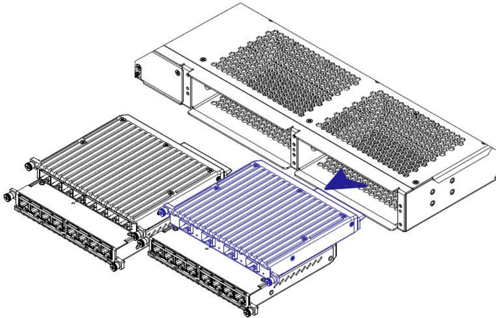
Figure 10: Removal of iRM-4TGSFP Module
