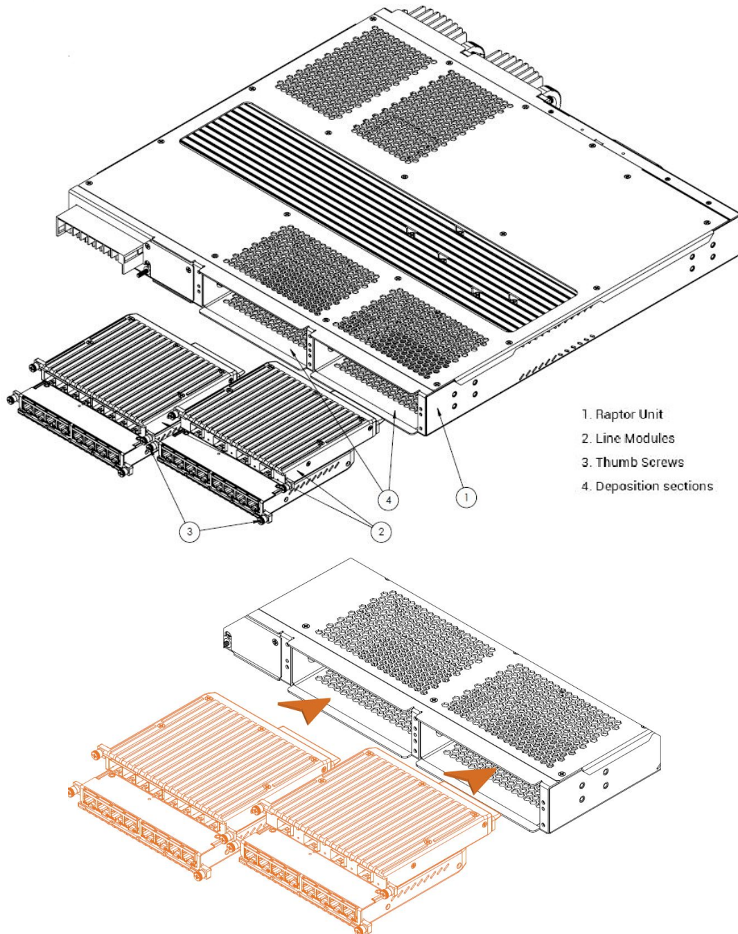
Figure 5: Line Modules Installation
