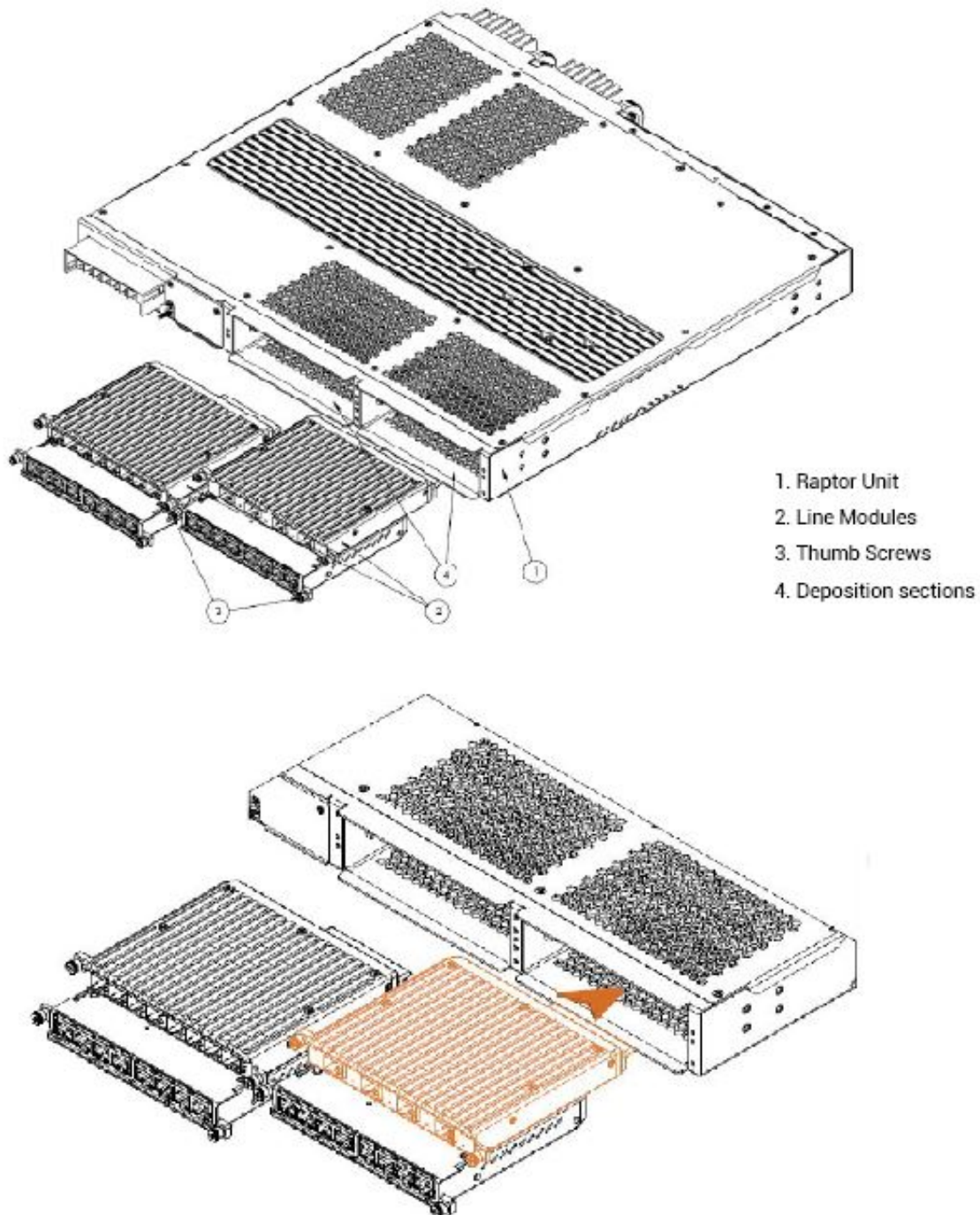
Figure 8: Removal of Line Modules from Chassis
