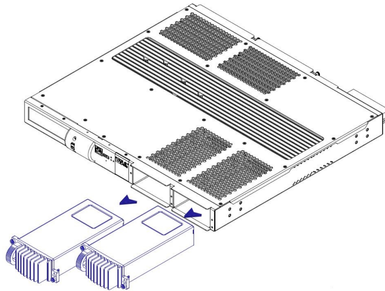
Figure 4: Removal of Power Supply Modules from Chassis
