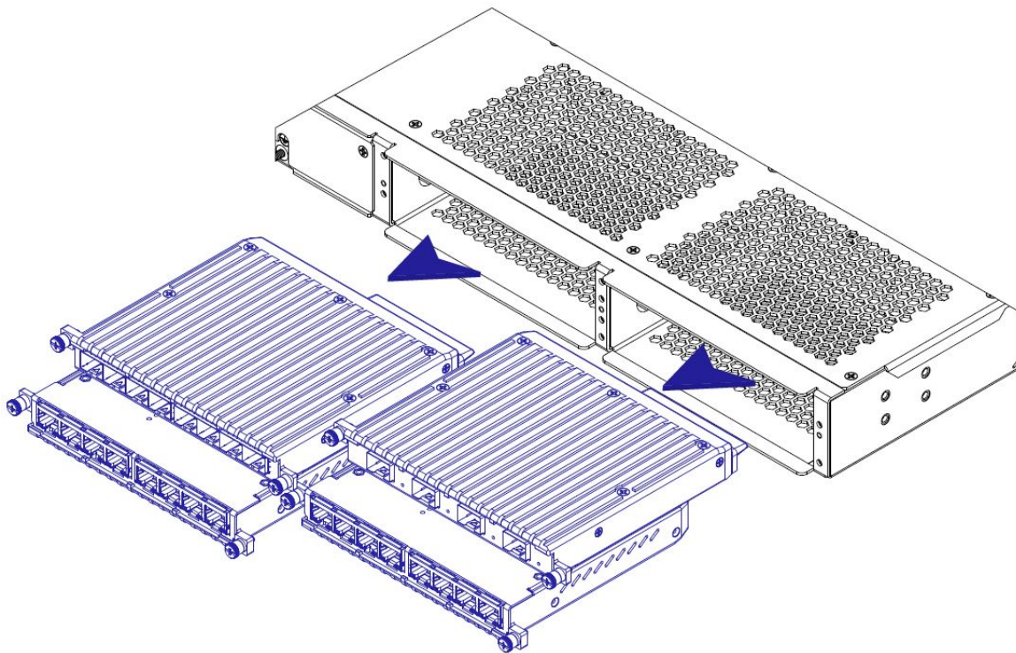
Figure 7: Removal of Line Modules from Chassis
