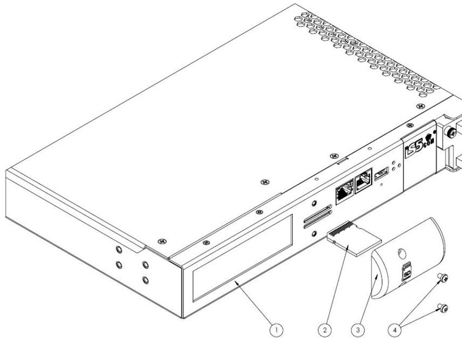
Figure 14: Removing SD Card
