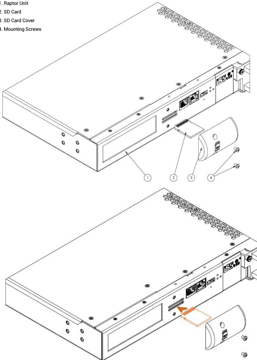
Figure 12: Inserting SD Card in SD Slot
