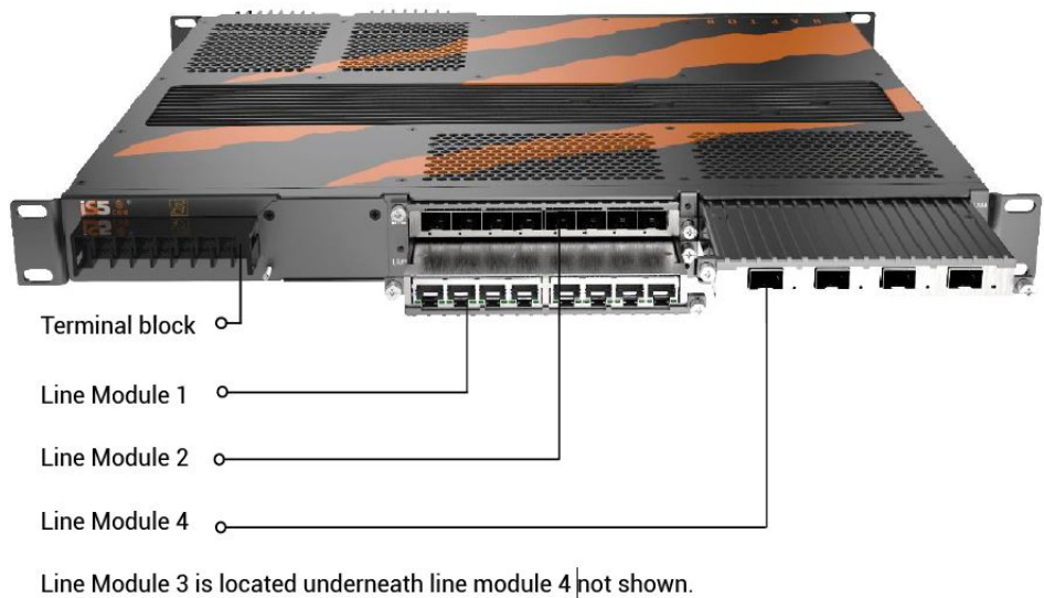
Figure 3: Back Panel Elements
