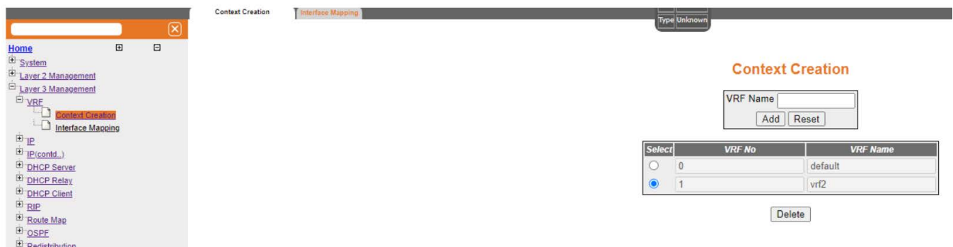
Figure 1: Context Creation
