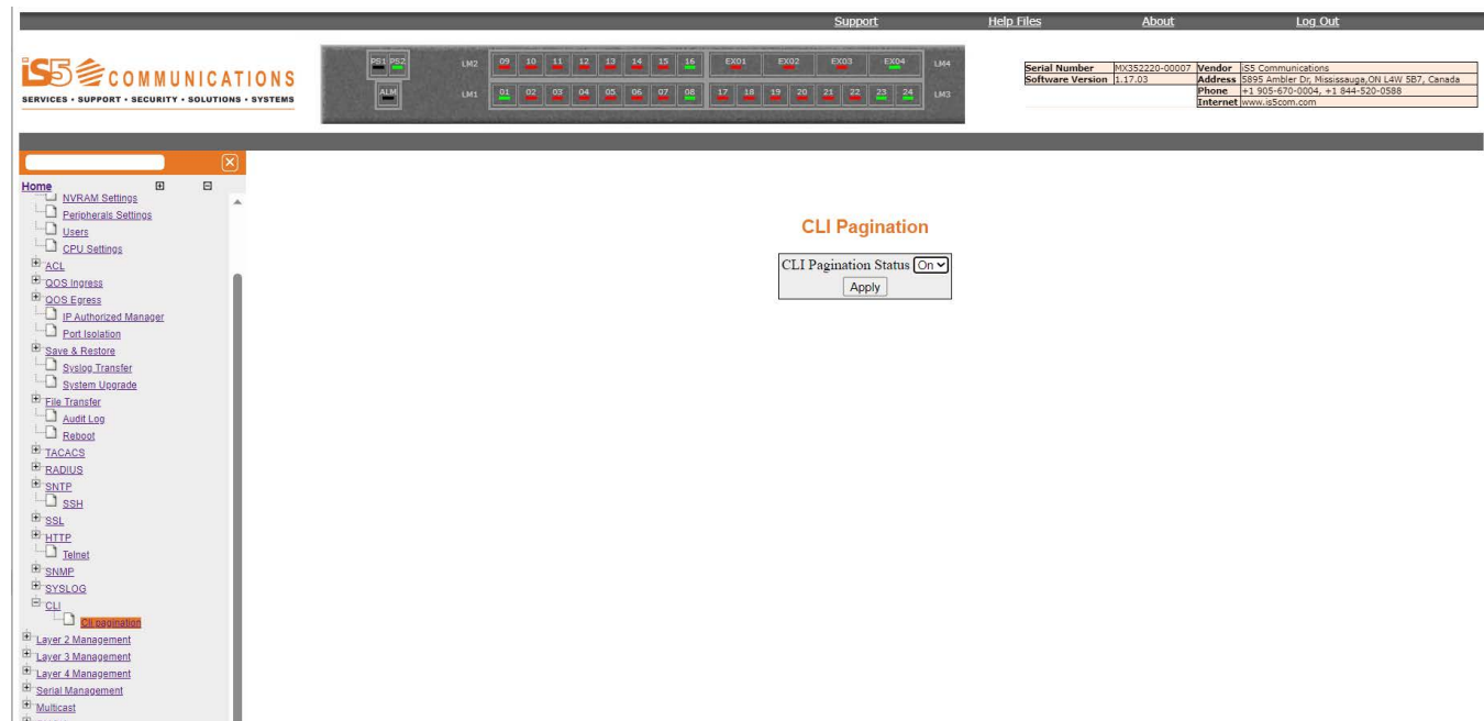
Figure 34: CLI Pagination
