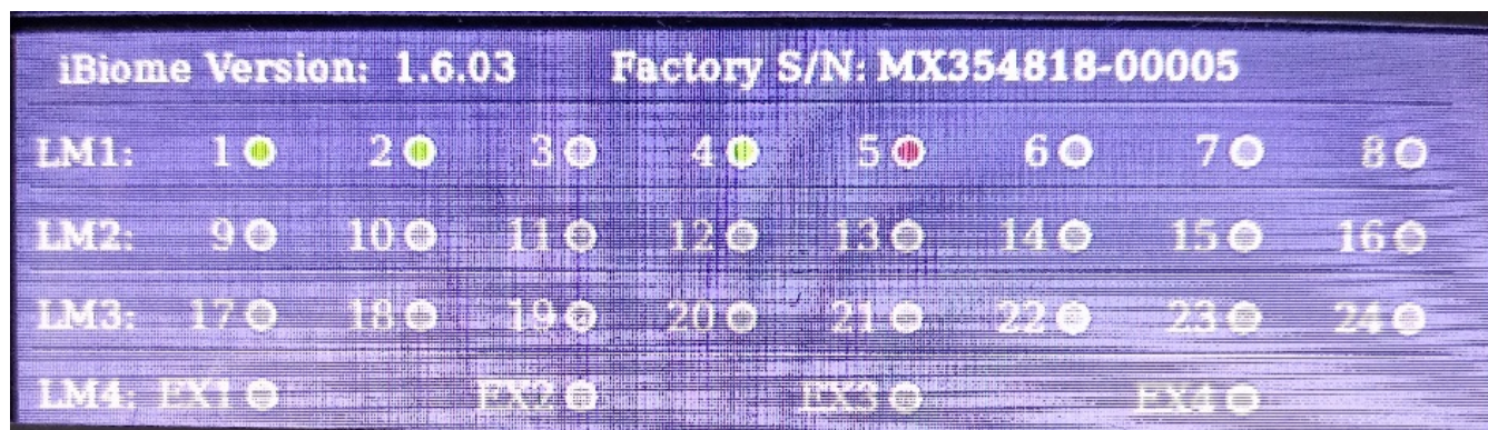
Figure 4: iMR350 LED Display
