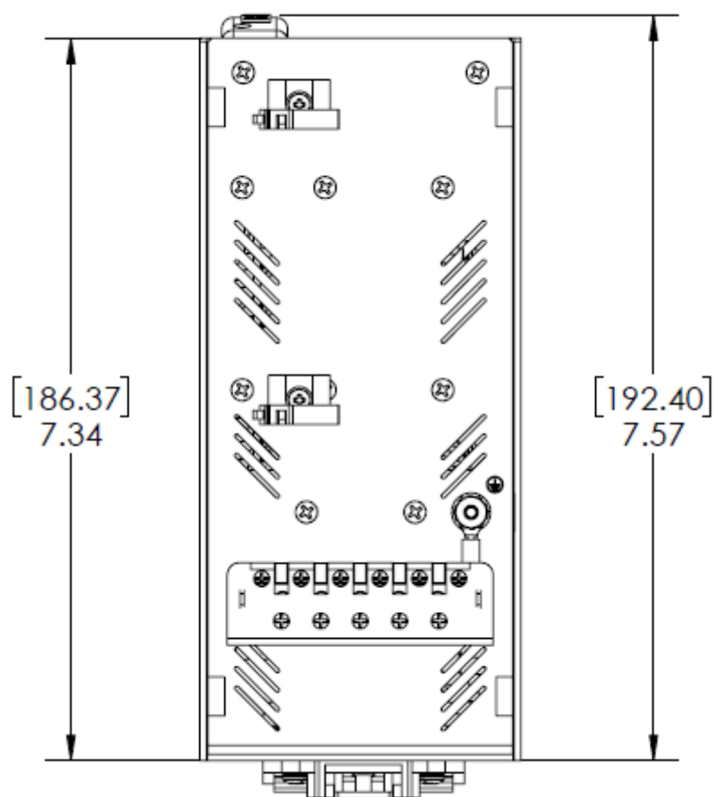
Figure 3: Bottom view of the iMR920
