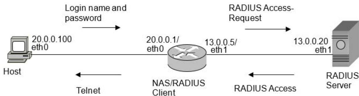
Figure 2: Packet Flow between Host, RADIUS CLIENT, and RADIUS server
