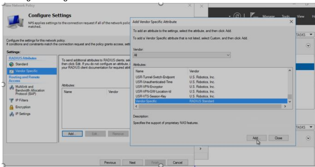
Figure 22: Configure Settings
