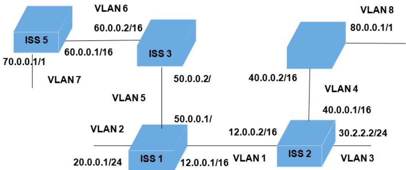
Figure 1: PIM- Testing Topology
