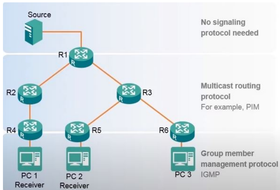
Figure 1: Multicast Distribution Tree
